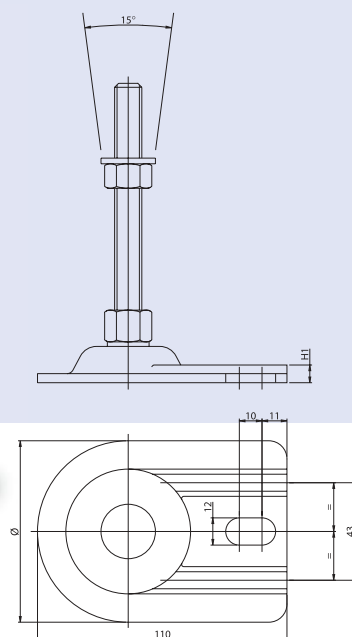
BSF80V
